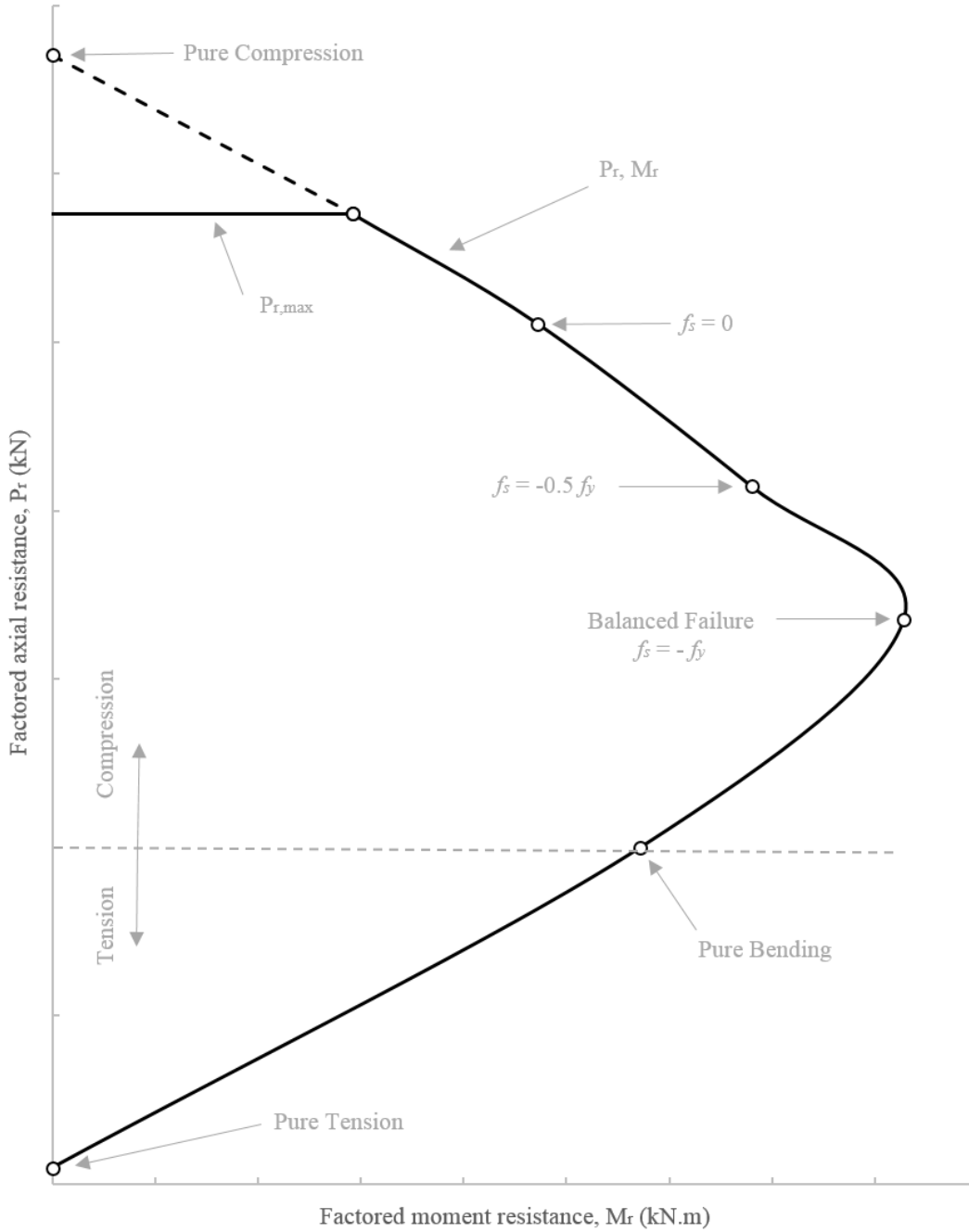
Figure 2 – Control Points
