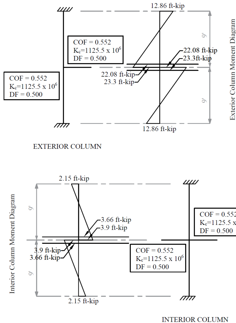
Figure 10a - Column Moments (Unbalanced Moments from Slab-Beam)
