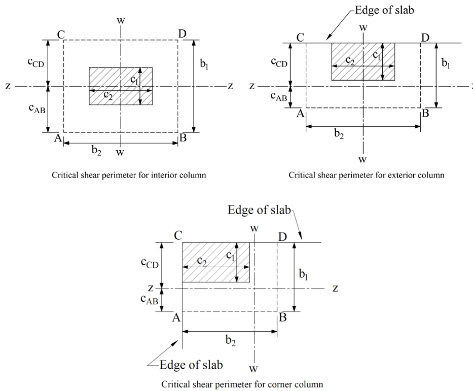
Figure 5 – Critical Shear Perimeters for Columns
