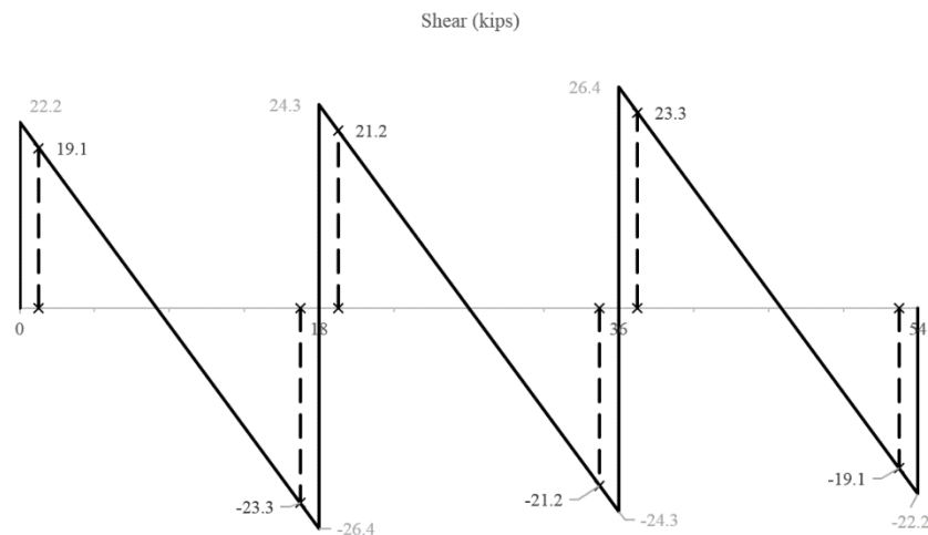
Figure 11 – One-way shear at critical sections (at distance d from the face of the supporting column)
