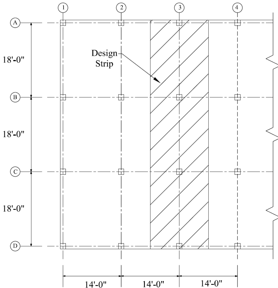
Figure 1 - Two-Way Flat Concrete Floor System
