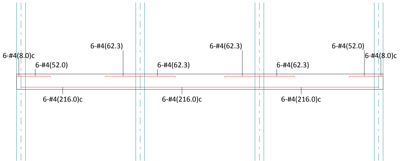
Middle Strip Flexural Reinforcement
