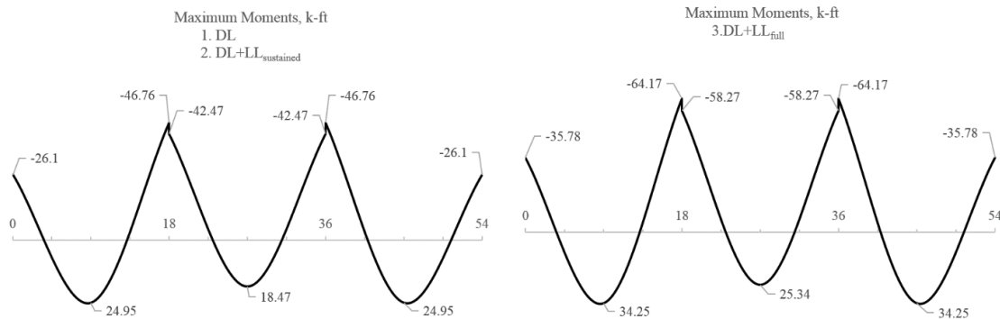
Figure 12 – Maximum Moments for the Three Service Load Levels
