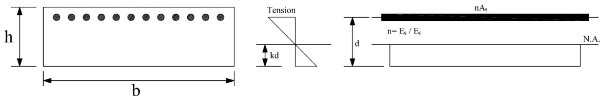
Figure 13 – Cracked Transformed Section
