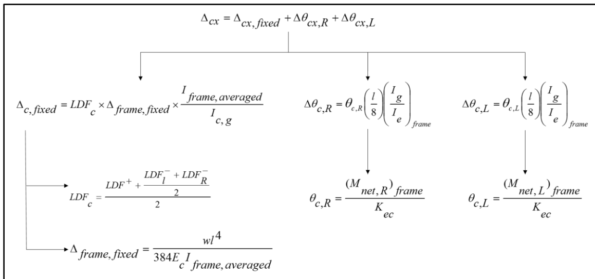
Figure 15 – \Delta_{cx} calculation procedure
