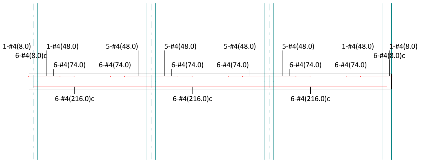
Column Strip Flexural Reinforcement
