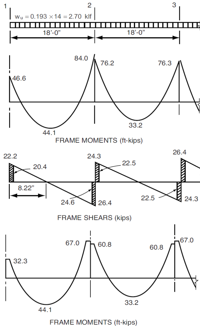
Figure 9 - Positive and Negative Design Moments for Slab-Beam (All Spans Loaded with Full Factored Live Load)
