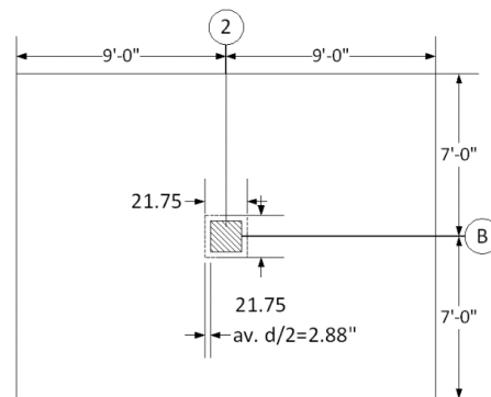
Figure 4 – Critical Section for Two-Way
