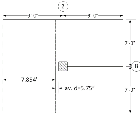
Figure 3 – Critical Section for One-Way
