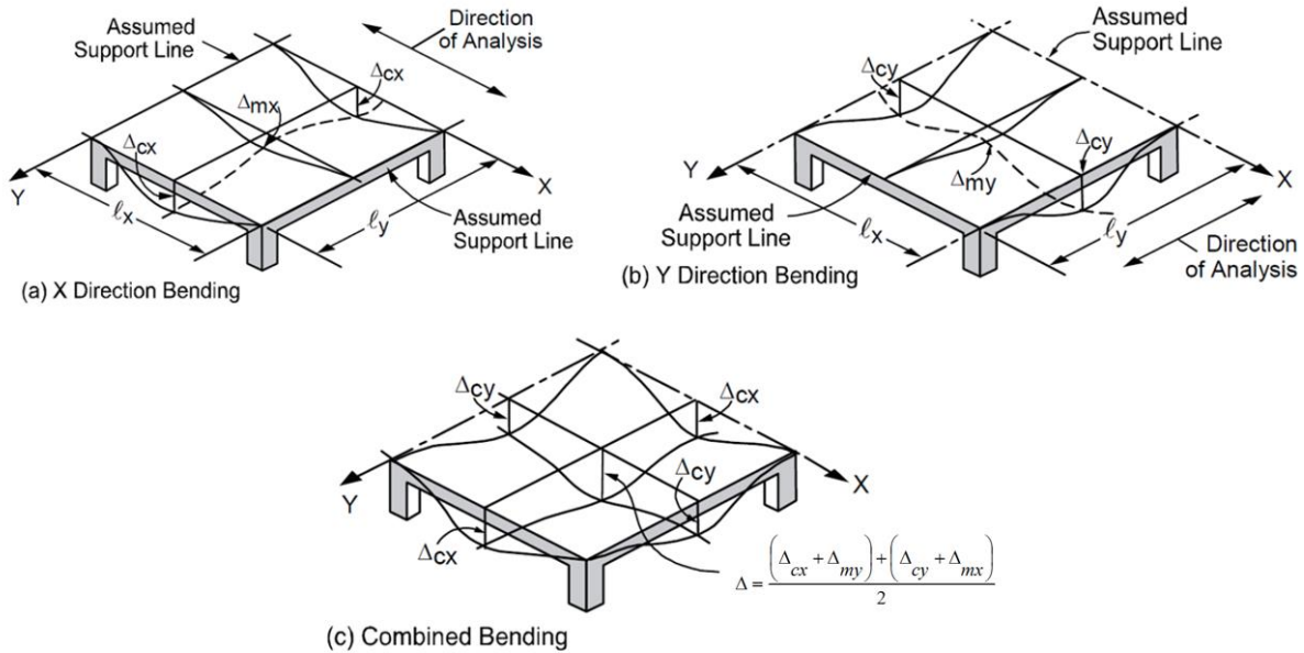
Figure 14 – Deflection Computation for a rectangular Panel
