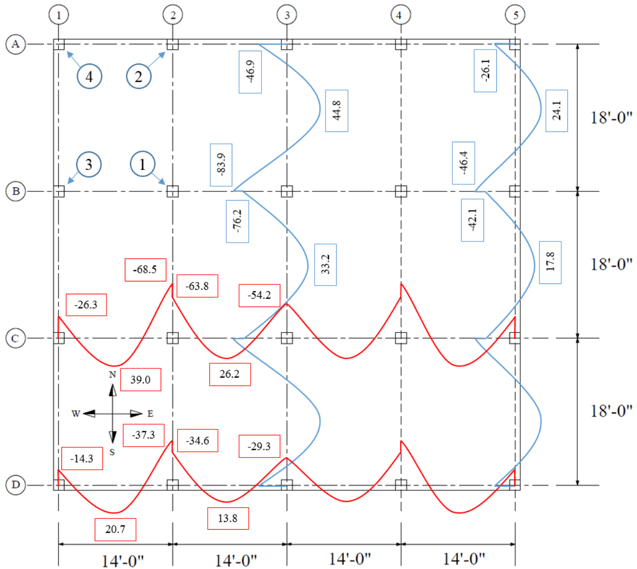
Figure 10b – Moment Diagrams (kips-ft)
