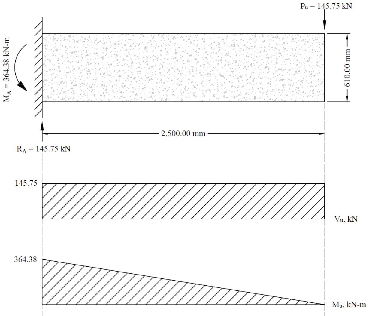
Figure 2 – Shear and Bending Moment Diagrams
