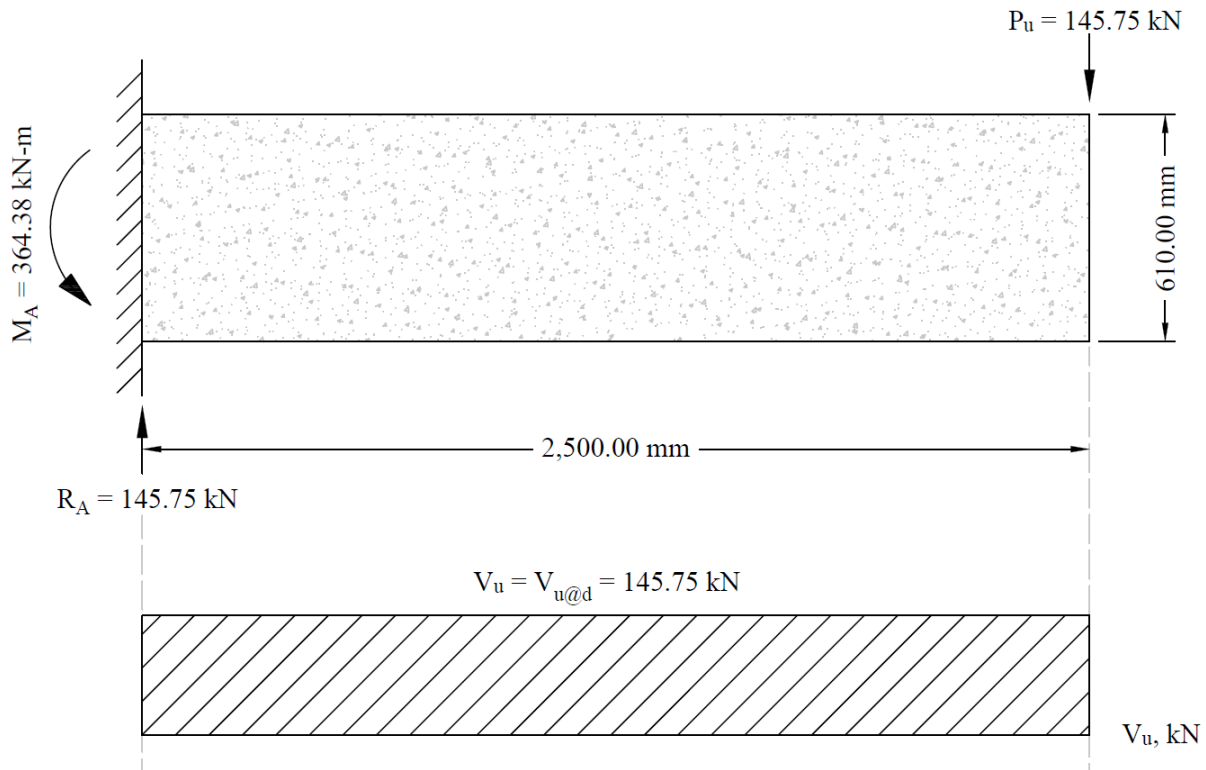
Figure 4 – Shear Diagram for Cantilever Beam
